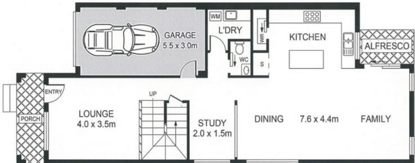
GROUND FLOOR
